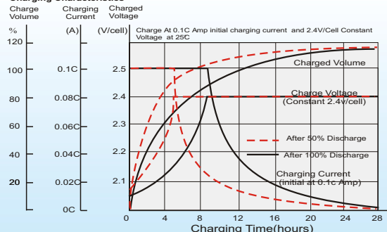
Charging Characteristics
